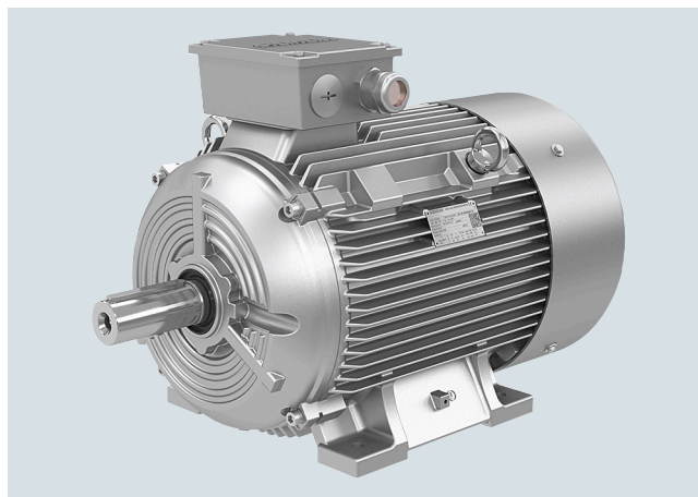
SIMOTICS 1LE0 with cast-iron housing, frame size 180
